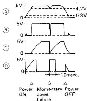
Fig. 14 Reset circuit and waveforms at respective points
