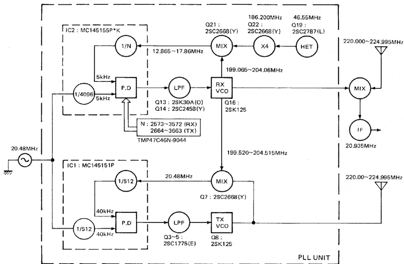
Fig. 7 Frequency-related block diagram
