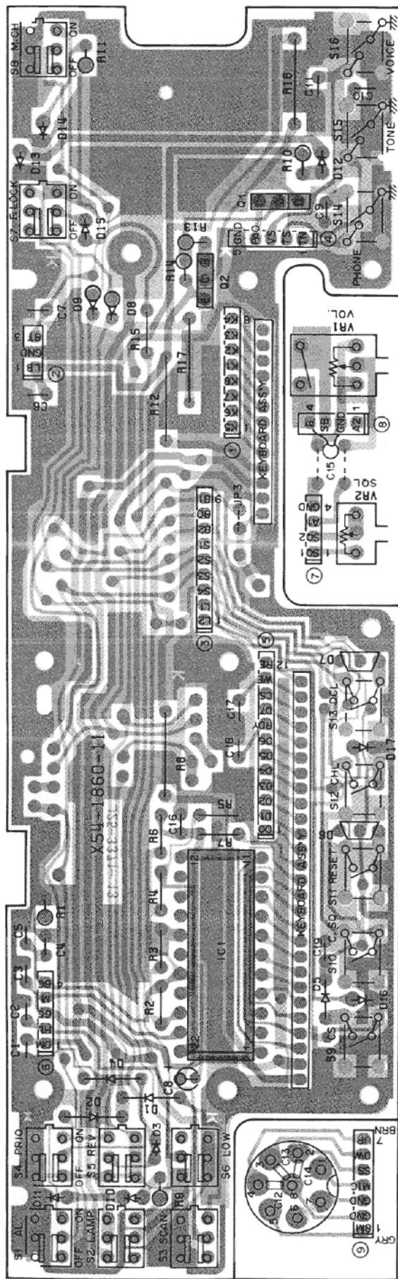
DISPLAY UNIT (X54-1860-11) Component side view
