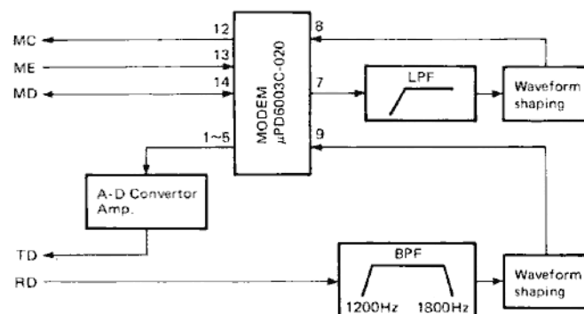
Fig. 16 MODEM unit (X57-1140-20) block diagram
