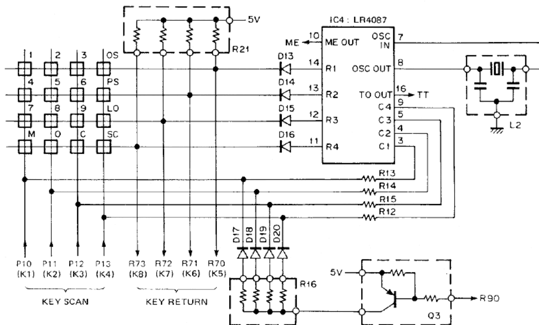
Fig. 11 DTMF circuit
