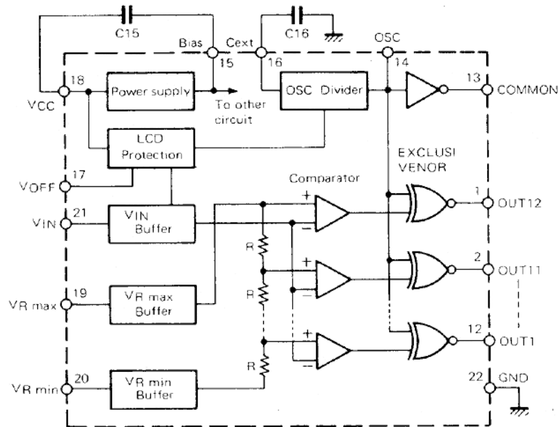
Fig. 18 IR2429 Block diagram (Display unit IC1)
