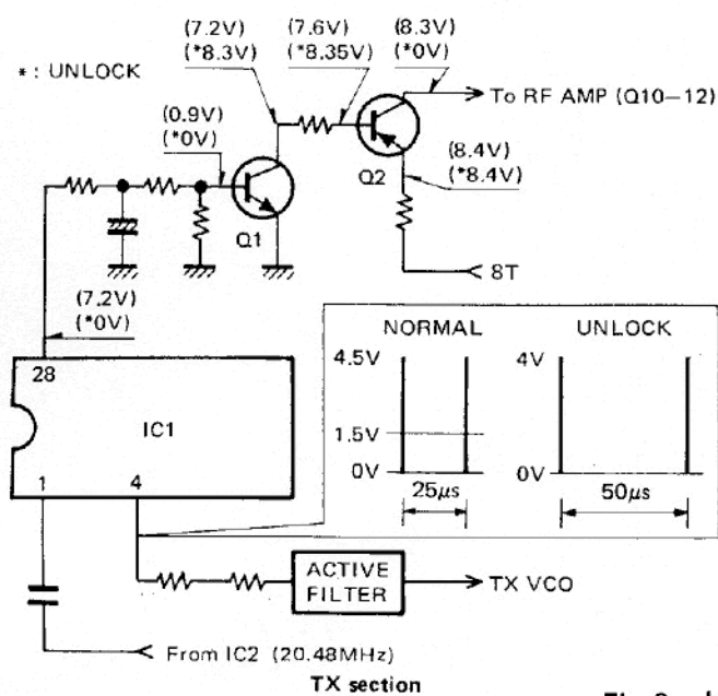
Fig. 8 Unlock circuit
