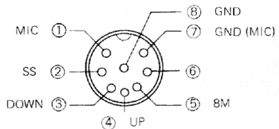
Fig. 19 MIC terminals (view from front panel side)
