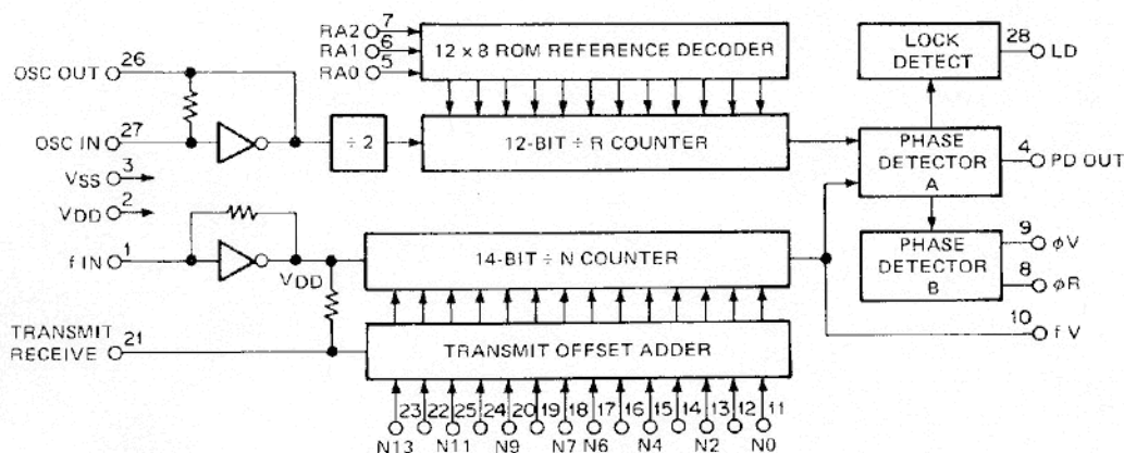
Fig. 6 MC145151P*J Block diagram (PLL unit IC1)
