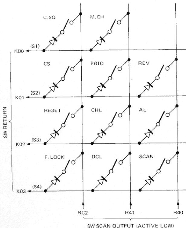
Fig. 9 Diode matrix
