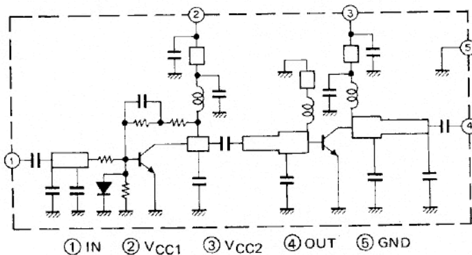
Fig. 4 M57774 Equivalent circuit
